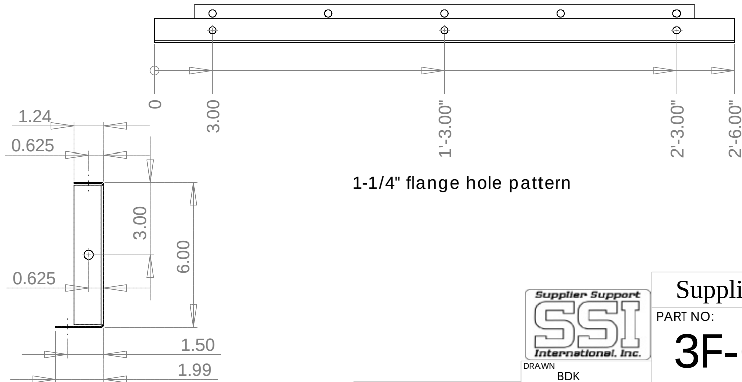
Side View [1:4]
